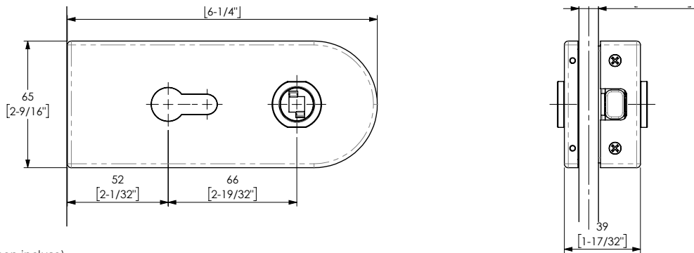
Claustra | 15910 Serratura magnetica Magnetic lock Cerradura magnetica
