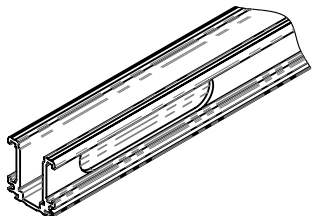
87801 Profilo WCP7 WCP7 Profile Perfil WCP7
